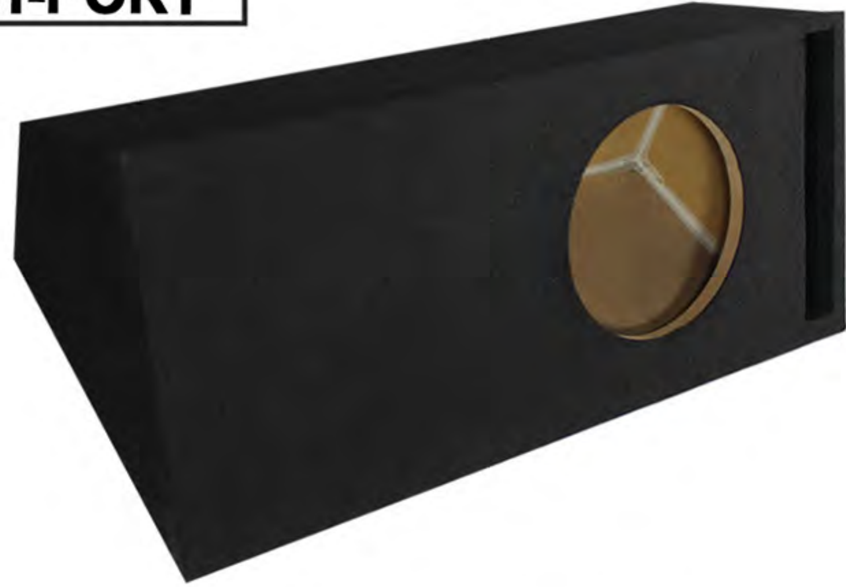
SINGLE SUB BOX (HATCHBACK) WITH A SINGLE PORT AVAILABLE SIZES: 8", 10", & 12"
